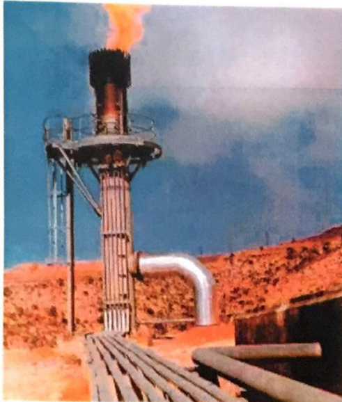
Figure 1 - Flare system at Kangan Phase1, satellite No.3 (Courtesy of Tehran Jonoub)
