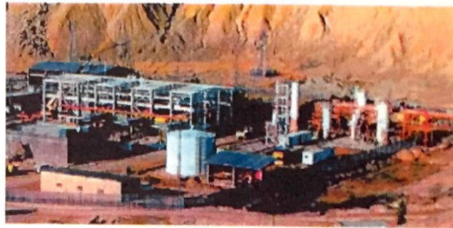
Figure 11 - Karanj Gas Injection Project (Courtesy of Sazeh Consultants)
