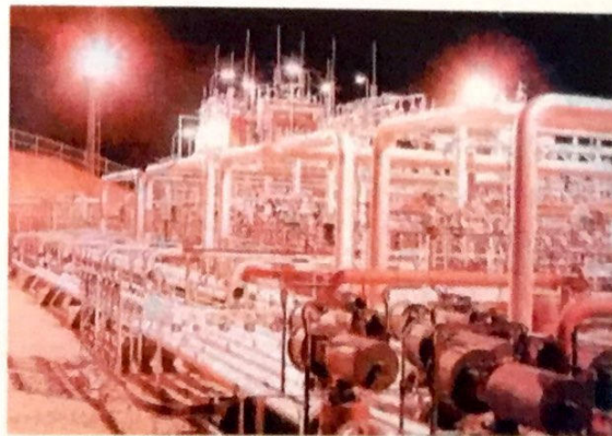
Figure 13 - Karanj Gas Injection Project Phase 1 (Courtesy of Tehran Jonoub)
